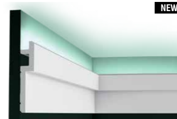
C395 STEPS 200 x 15,5 x 3,1 cm Purotouch® Designed by Orio Tonini
