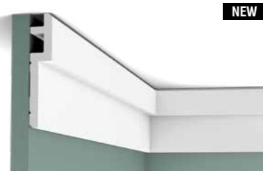
C395 STEPS 200 x 15,5 x 3,1 cm Purotouch® Designed by Orio Tonini
